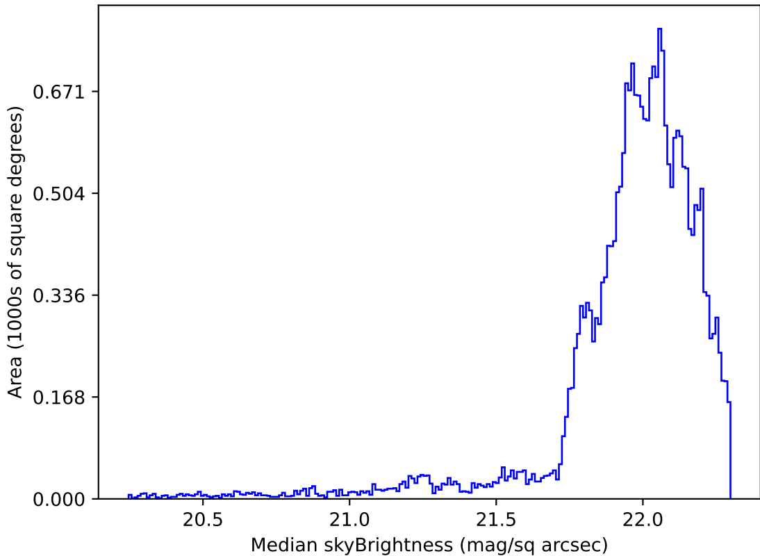
too_elab_r16_d3_giz_v3.4_10yrs Yr 1 g band: Median skyBrightness
