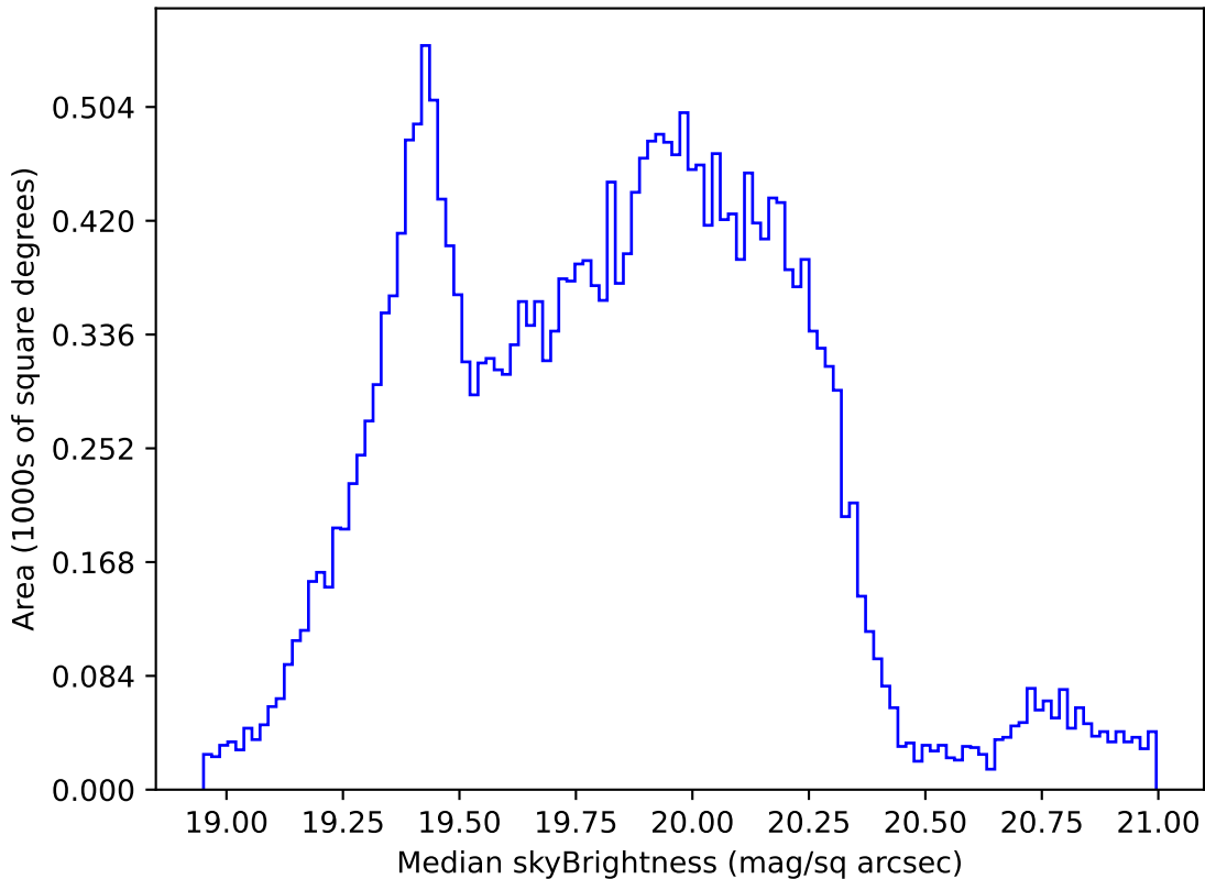
too_elab_r16_d3_giz_v3.4_10yrs Yr 1 all bands: Median skyBrightness
