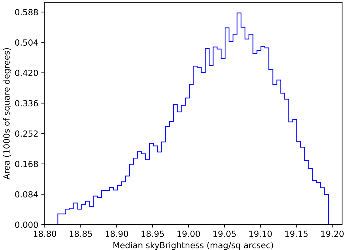
too_elab_r16_d3_giz_v3.4_10yrs WFD z band: Median skyBrightness
