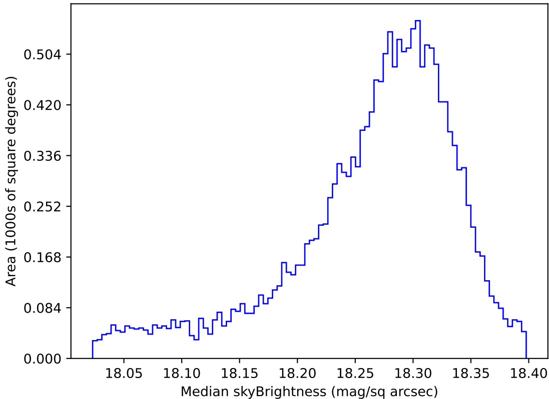
too_elab_r16_d3_giz_v3.4_10yrs WFD y band: Median skyBrightness
