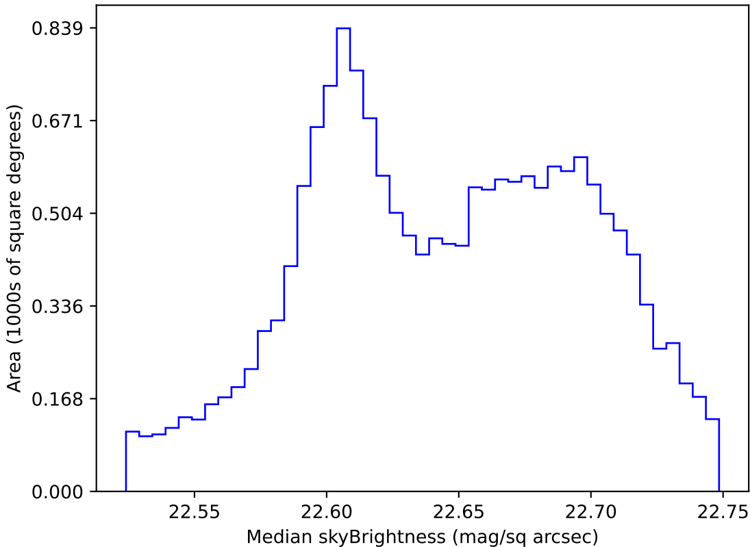
too_elab_r16_d3_giz_v3.4_10yrs WFD u band: Median skyBrightness
