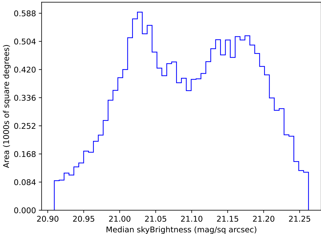
too_elab_r16_d3_giz_v3.4_10yrs WFD r band: Median skyBrightness
