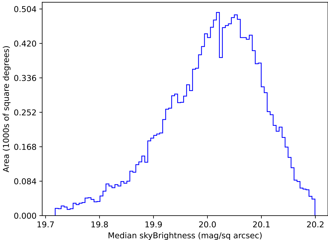
too_elab_r16_d3_giz_v3.4_10yrs WFD i band: Median skyBrightness
