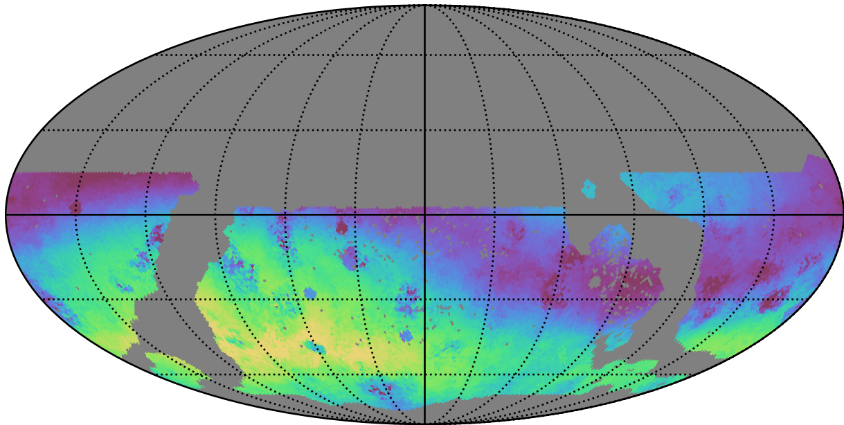
too_elab_r16_d3_giz_v3.4_10yrs WFD g band: Median skyBrightness
