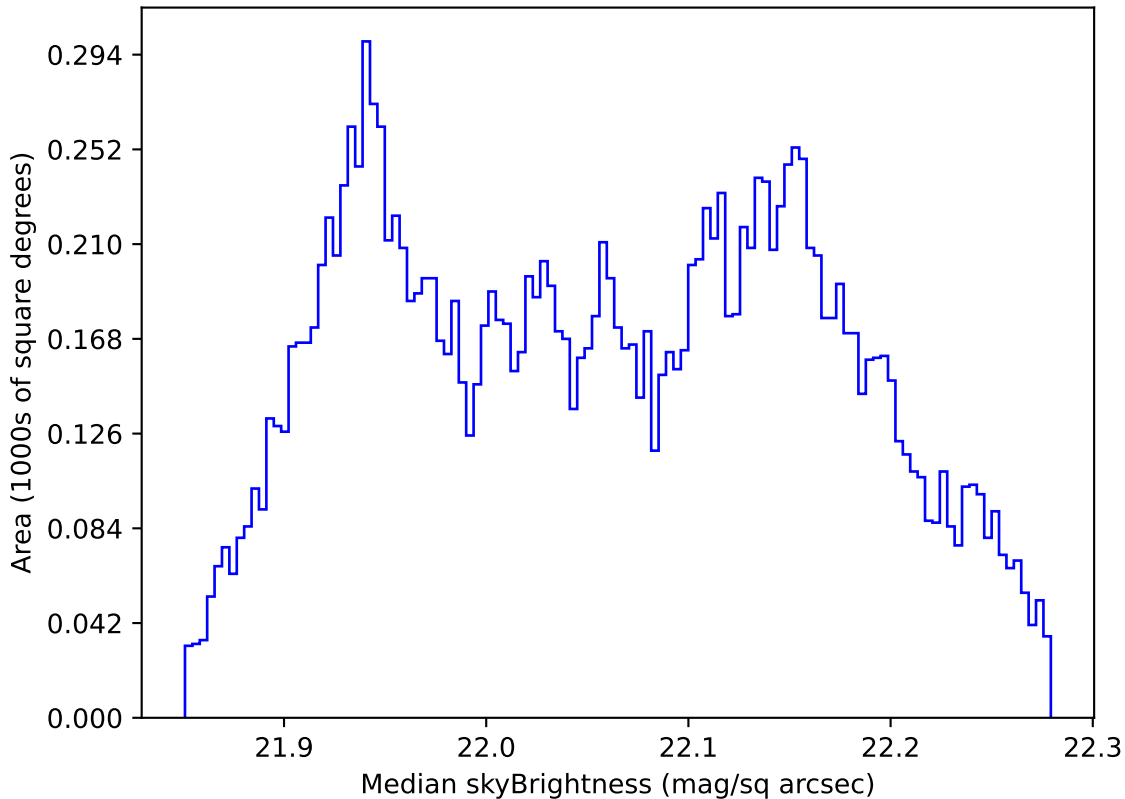
too_elab_r16_d3_giz_v3.4_10yrs WFD g band: Median skyBrightness
