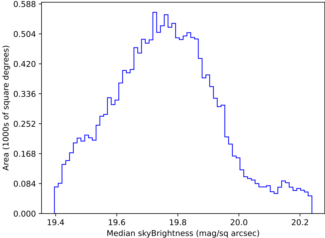
too_elab_r16_d3_giz_v3.4_10yrs WFD all bands: Median skyBrightness
