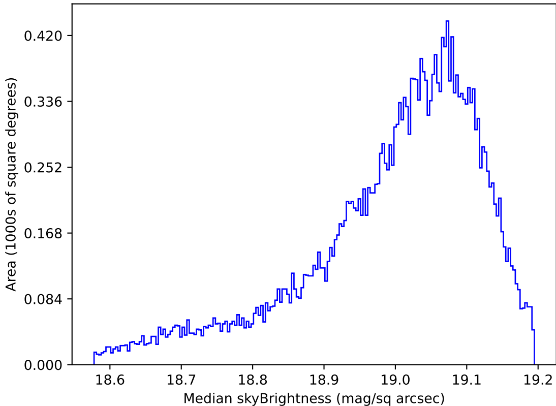
too_elab_r16_d3_giz_v3.4_10yrs All sky z band: Median skyBrightness
