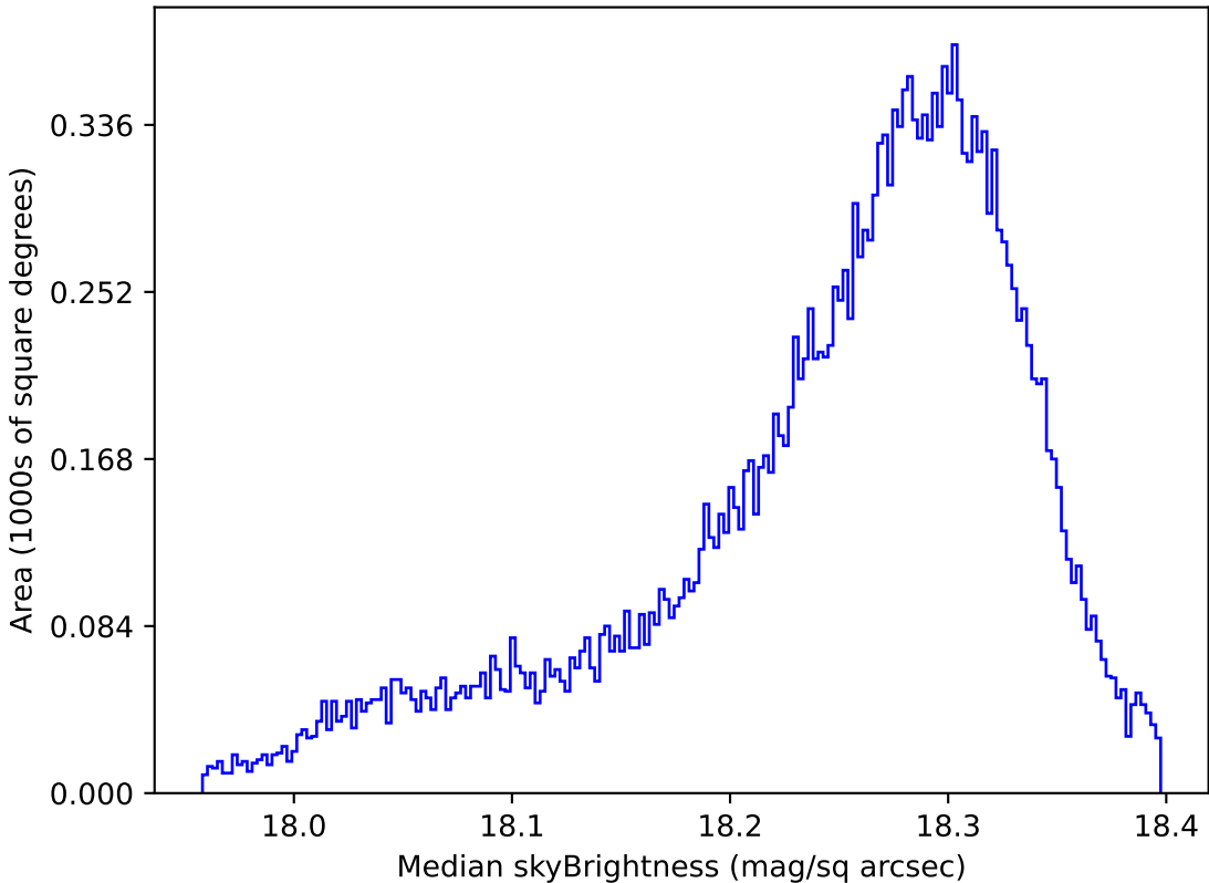
too_elab_r16_d3_giz_v3.4_10yrs All sky y band: Median skyBrightness
