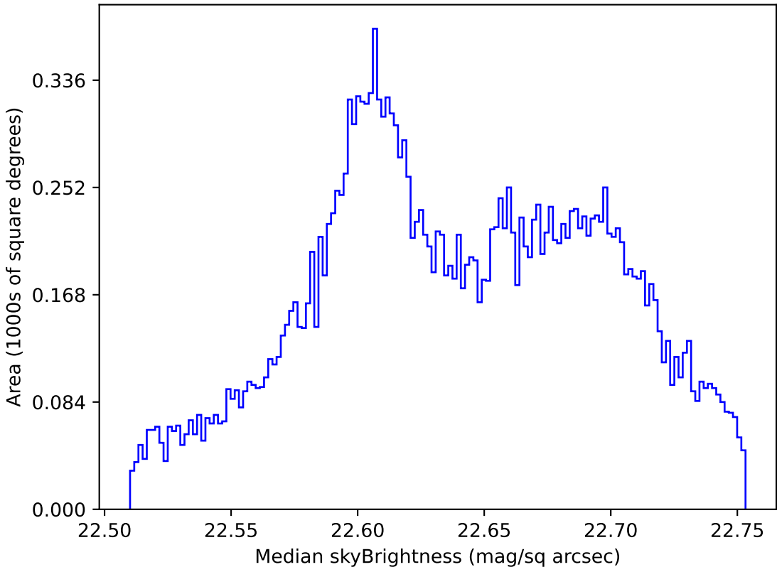
too_elab_r16_d3_giz_v3.4_10yrs All sky u band: Median skyBrightness
