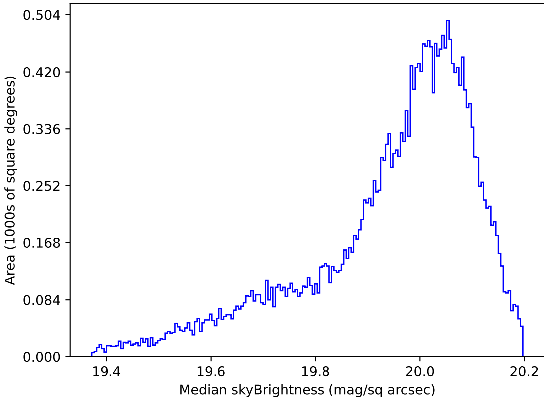
too_elab_r16_d3_giz_v3.4_10yrs All sky i band: Median skyBrightness
