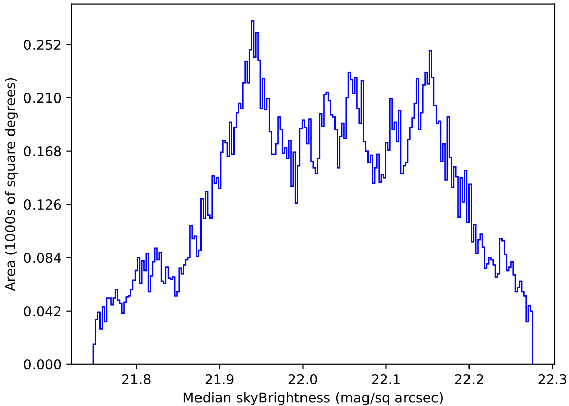
too_elab_r16_d3_giz_v3.4_10yrs All sky g band: Median skyBrightness
