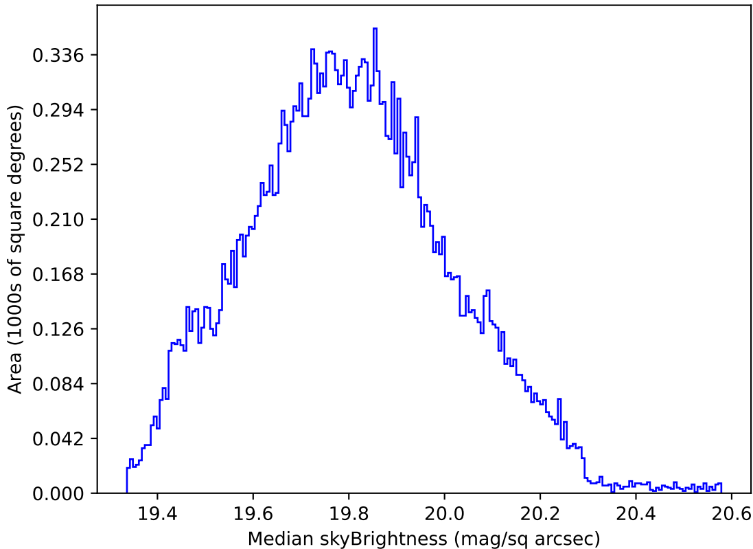
too_elab_r16_d3_giz_v3.4_10yrs All sky all bands: Median skyBrightness
