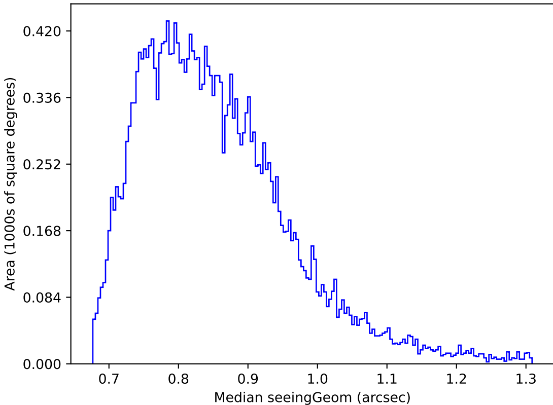
too_elab_r16_d3_giz_v3.4_10yrs Yr 1 z band: Median seeingGeom
