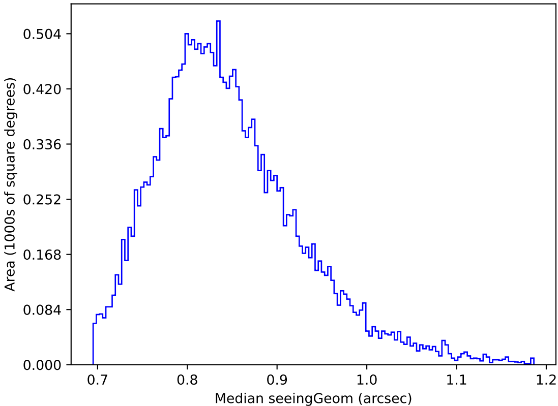
too_elab_r16_d3_giz_v3.4_10yrs Yr 1 y band: Median seeingGeom
