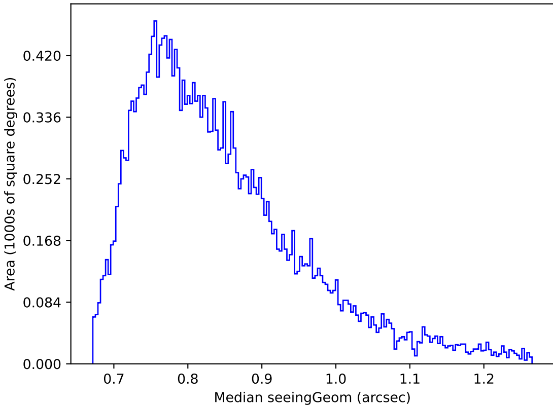
too_elab_r16_d3_giz_v3.4_10yrs Yr 1 i band: Median seeingGeom
