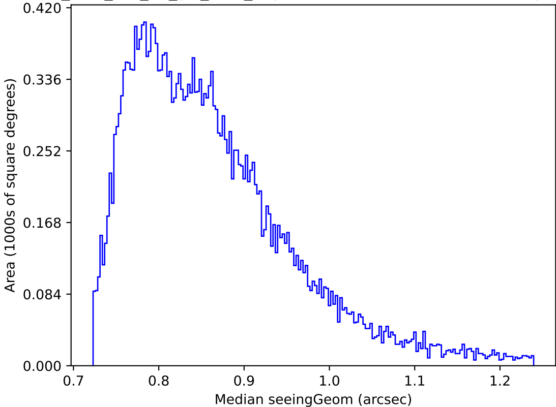
too_elab_r16_d3_giz_v3.4_10yrs Yr 1 all bands: Median seeingGeom
