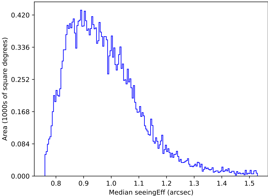
too_elab_r16_d3_giz_v3.4_10yrs Yr 1 z band: Median seeingEff
