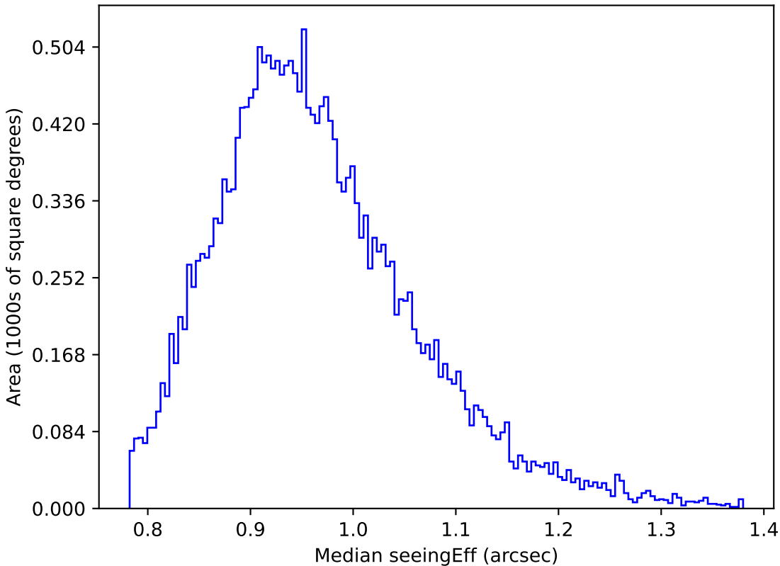
too_elab_r16_d3_giz_v3.4_10yrs Yr 1 y band: Median seeingEff
