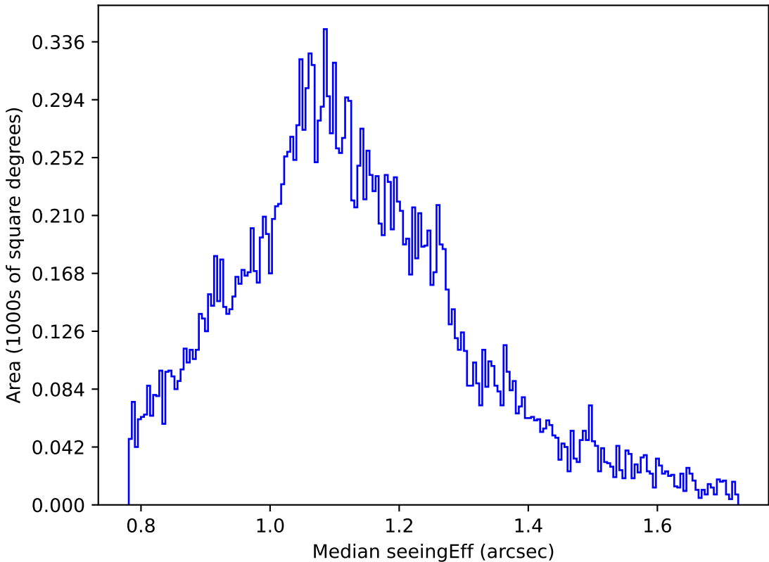
too_elab_r16_d3_giz_v3.4_10yrs Yr 1 u band: Median seeingEff
