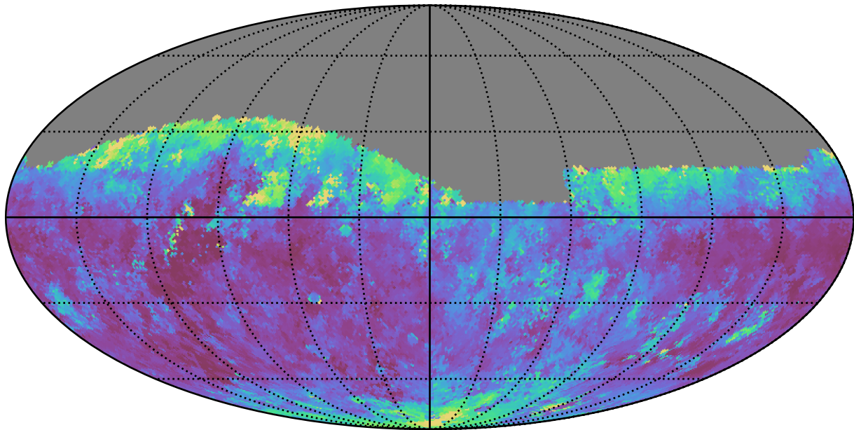
too_elab_r16_d3_giz_v3.4_10yrs Yr 1 r band: Median seeingEff
