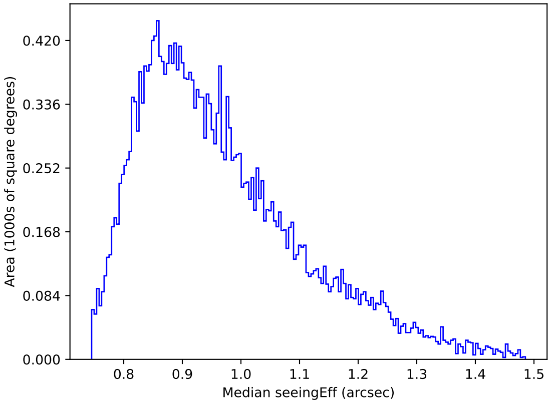
too_elab_r16_d3_giz_v3.4_10yrs Yr 1 r band: Median seeingEff
