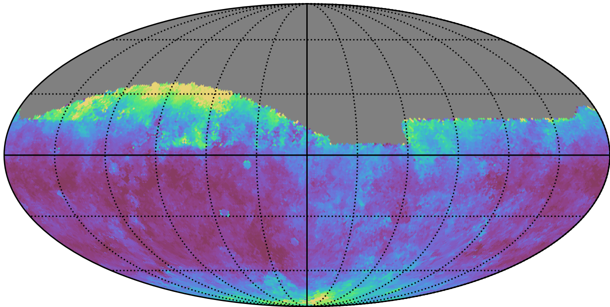
too_elab_r16_d3_giz_v3.4_10yrs Yr 1 all bands: Median seeingEff
