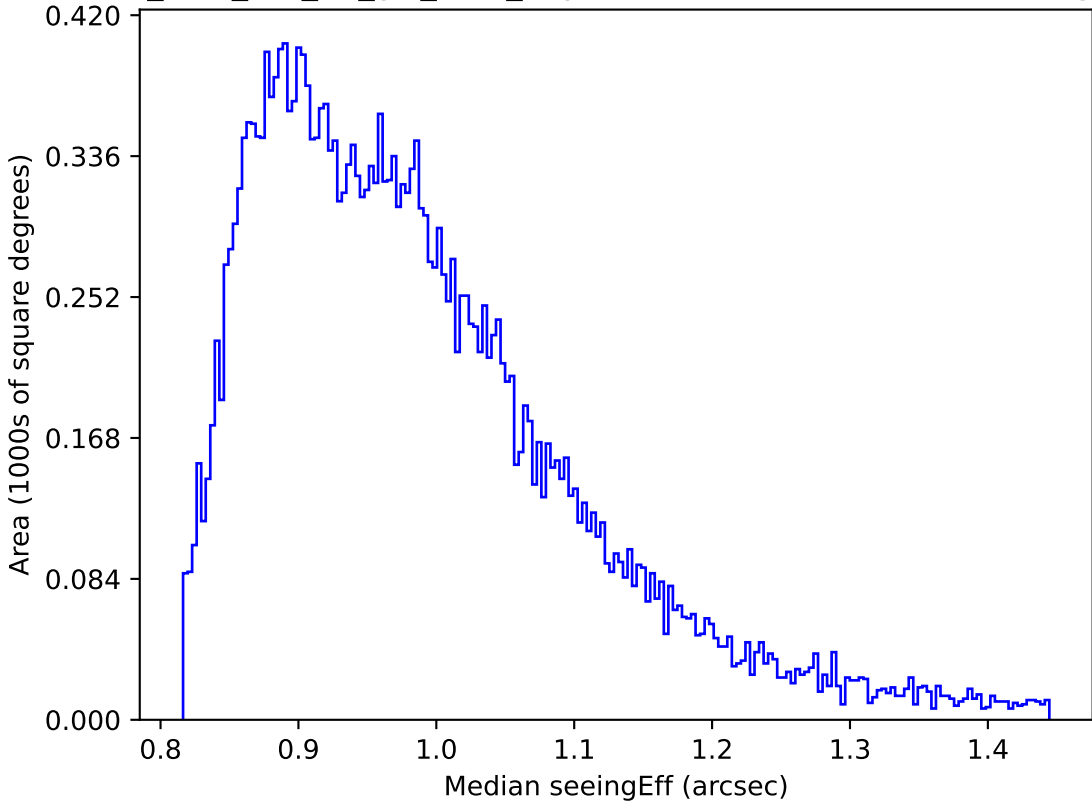
too_elab_r16_d3_giz_v3.4_10yrs Yr 1 all bands: Median seeingEff
