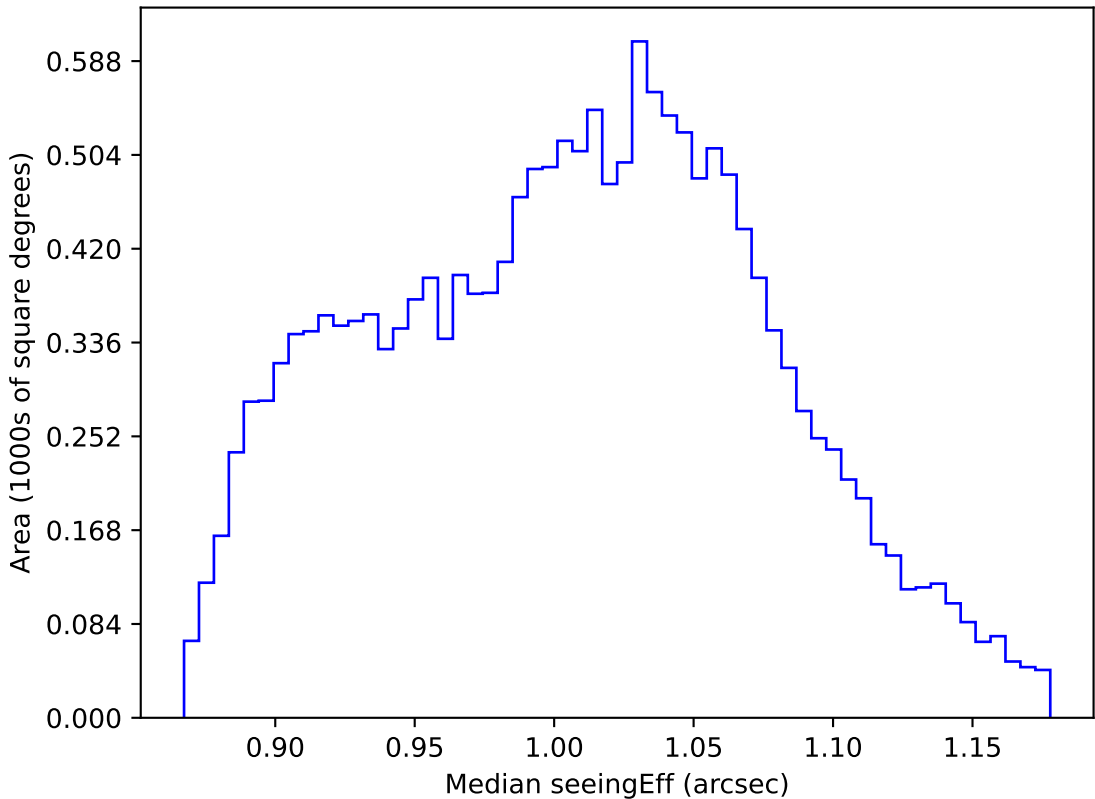
too_elab_r16_d3_giz_v3.4_10yrs WFD z band: Median seeingEff
