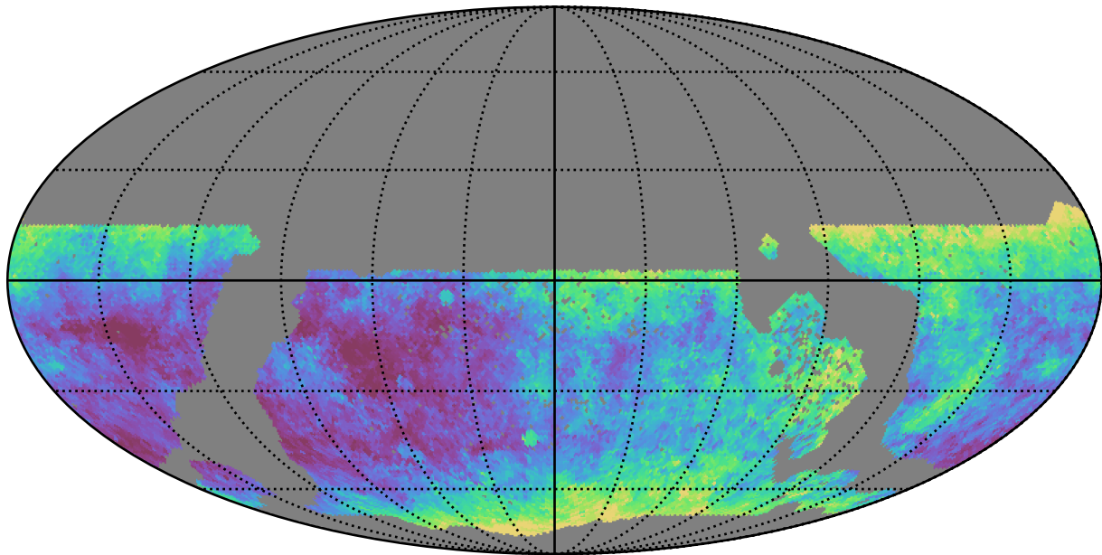
too_elab_r16_d3_giz_v3.4_10yrs WFD y band: Median seeingEff
