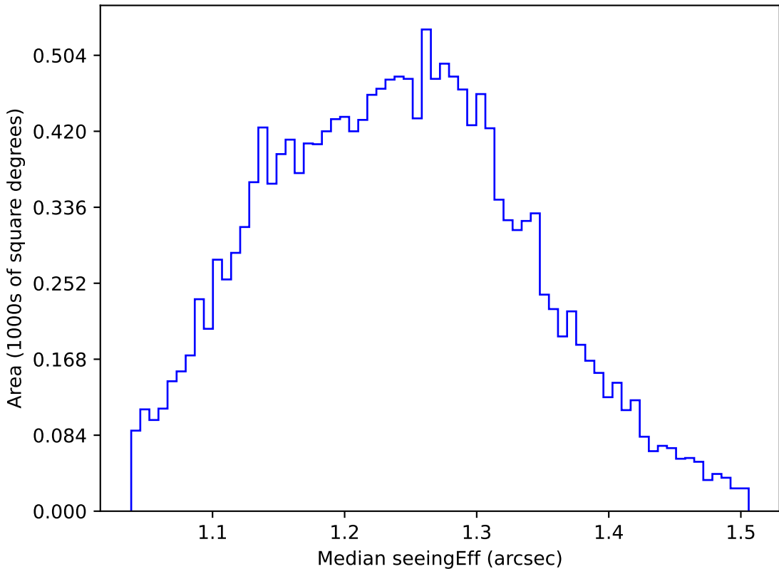
too_elab_r16_d3_giz_v3.4_10yrs WFD u band: Median seeingEff
