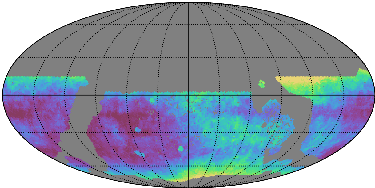
too_elab_r16_d3_giz_v3.4_10yrs WFD r band: Median seeingEff
