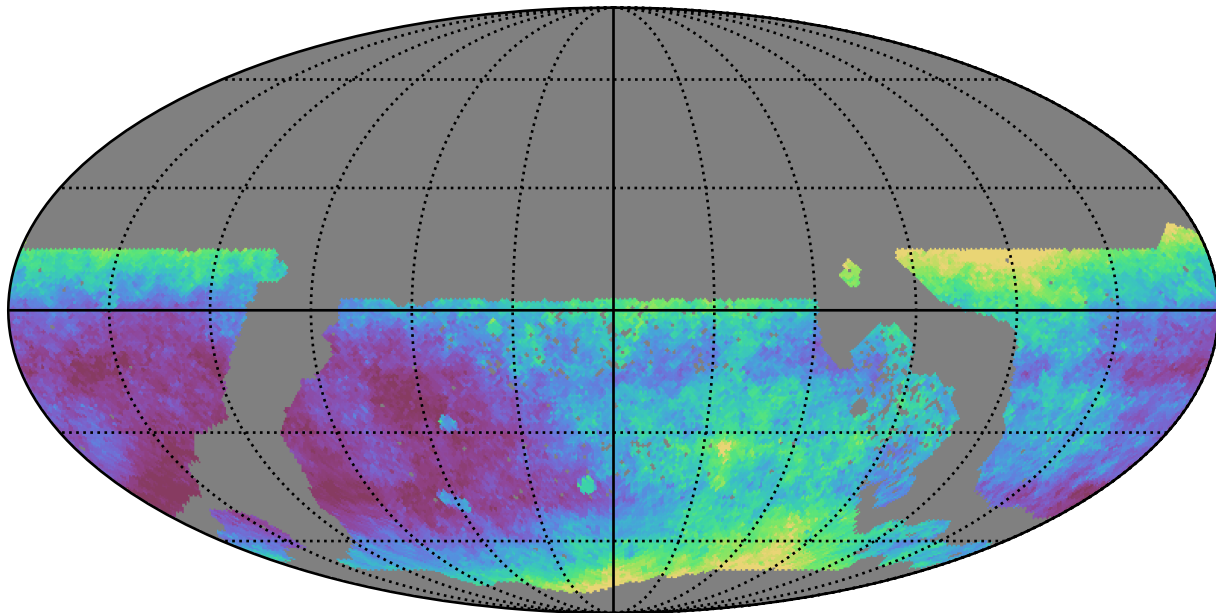
too_elab_r16_d3_giz_v3.4_10yrs WFD i band: Median seeingEff
