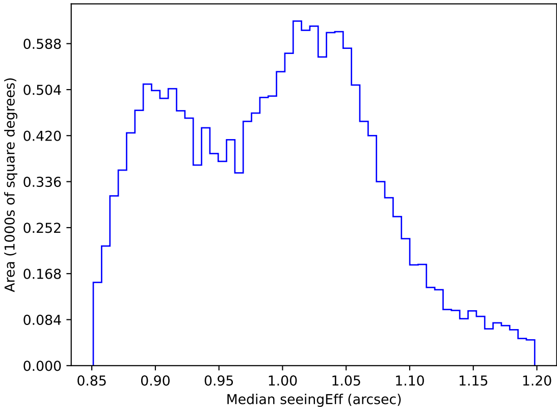
too_elab_r16_d3_giz_v3.4_10yrs WFD i band: Median seeingEff
