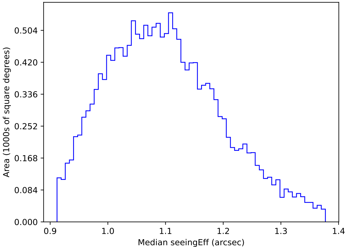
too_elab_r16_d3_giz_v3.4_10yrs WFD g band: Median seeingEff
