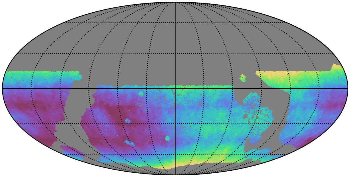
too_elab_r16_d3_giz_v3.4_10yrs WFD all bands: Median seeingEff
