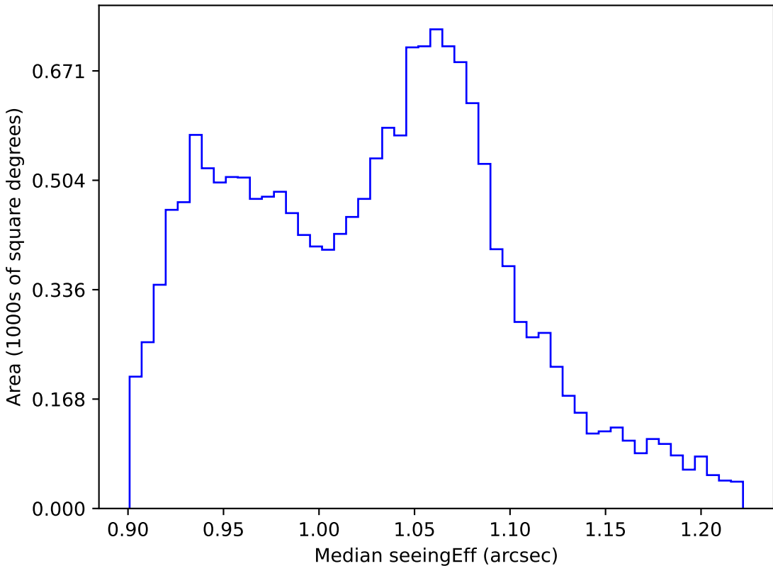
too_elab_r16_d3_giz_v3.4_10yrs WFD all bands: Median seeingEff
