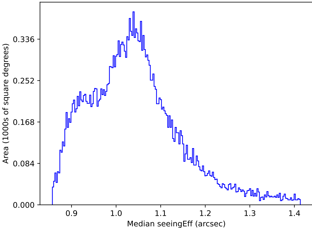
too_elab_r16_d3_giz_v3.4_10yrs All sky z band: Median seeingEff
