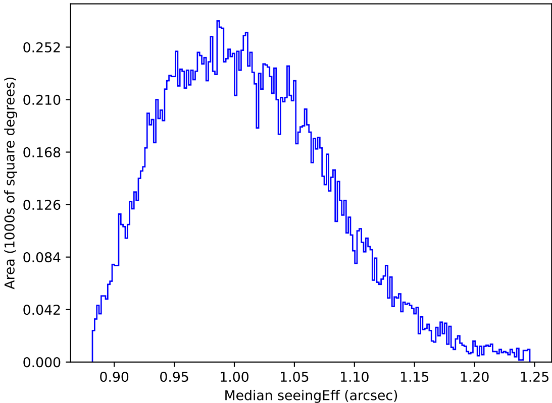
too_elab_r16_d3_giz_v3.4_10yrs All sky y band: Median seeingEff
