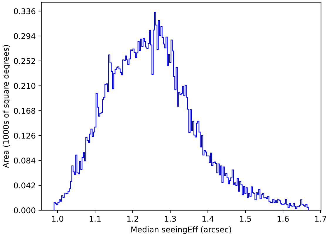
too_elab_r16_d3_giz_v3.4_10yrs All sky u band: Median seeingEff
