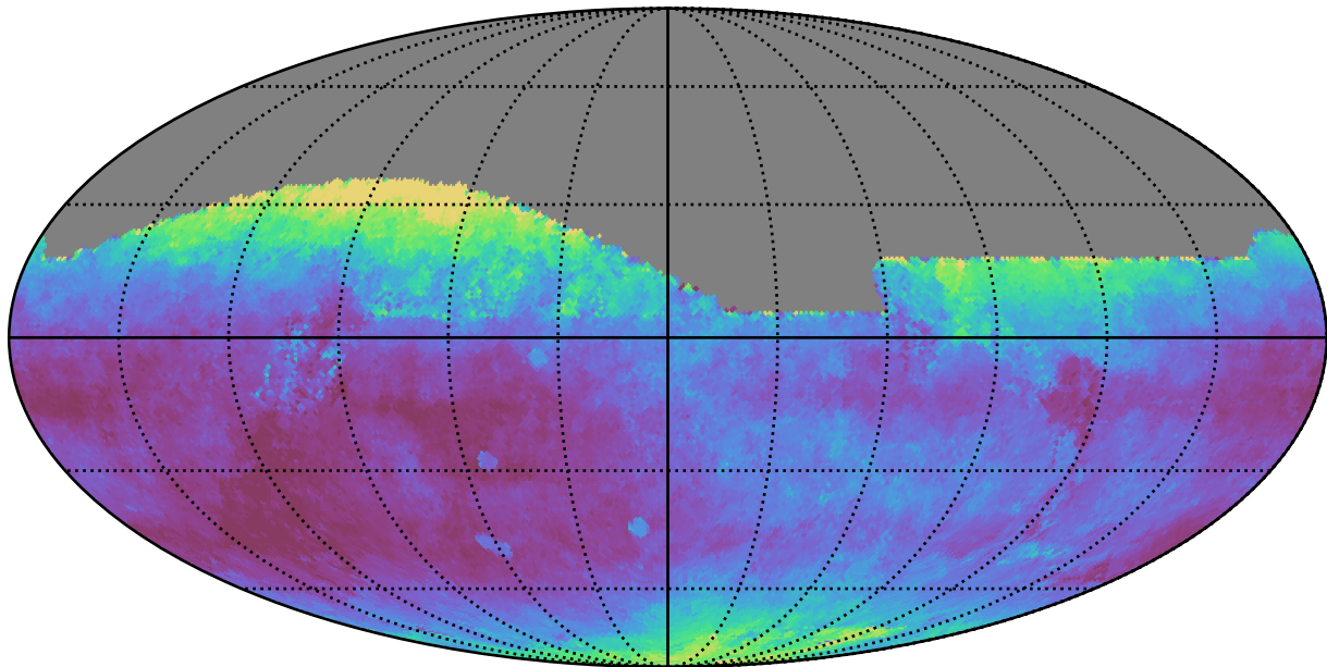
too_elab_r16_d3_giz_v3.4_10yrs All sky r band: Median seeingEff
