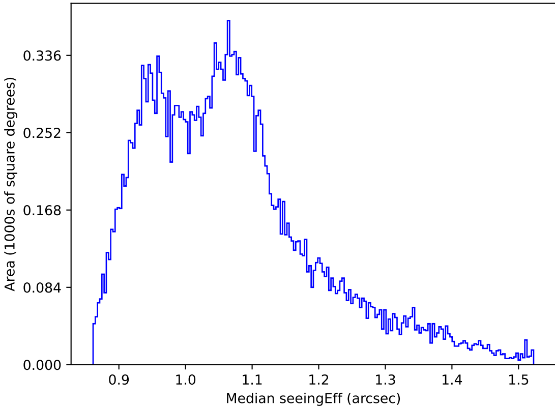
too_elab_r16_d3_giz_v3.4_10yrs All sky r band: Median seeingEff
