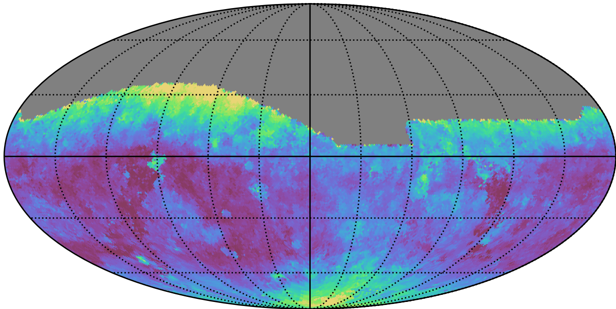
too_elab_r16_d3_giz_v3.4_10yrs All sky g band: Median seeingEff
