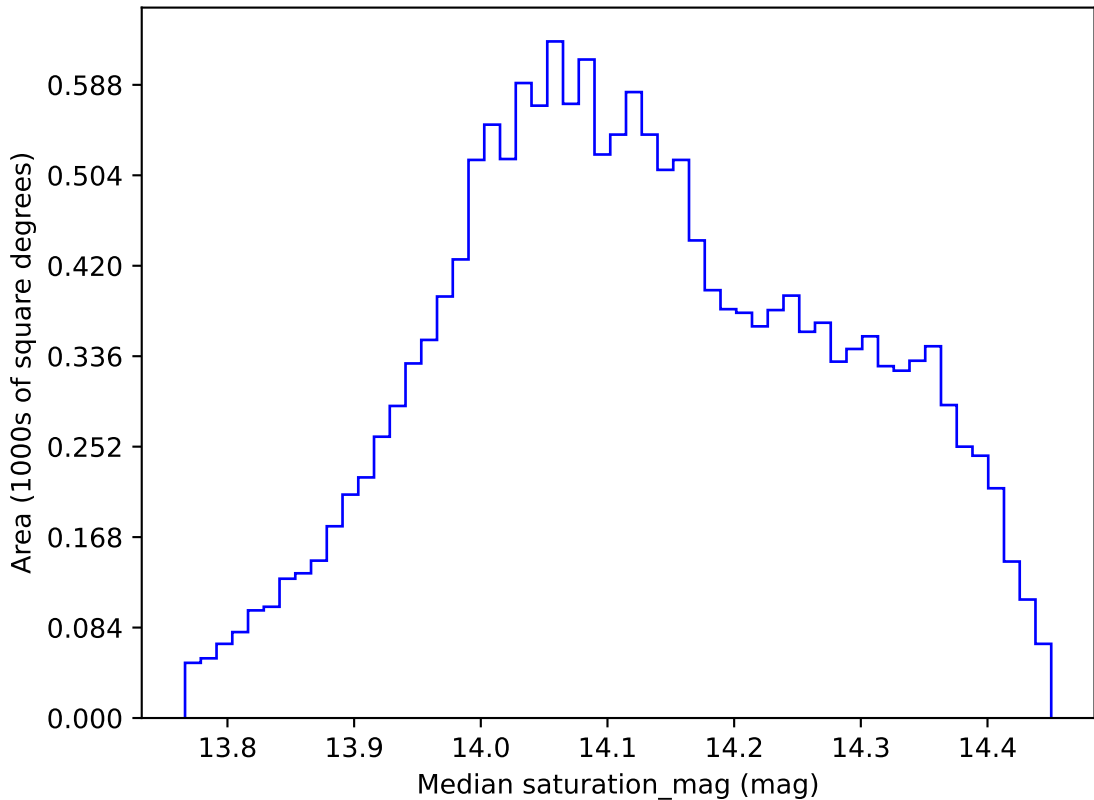
too_elab_r16_d3_giz_v3.4_10yrs WFD z band: Median saturation_mag
