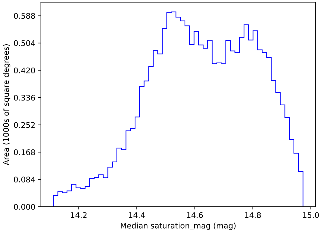
too_elab_r16_d3_giz_v3.4_10yrs WFD r band: Median saturation_mag
