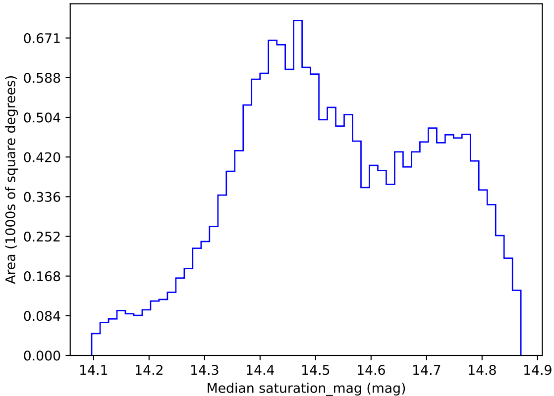
too_elab_r16_d3_giz_v3.4_10yrs WFD i band: Median saturation_mag
