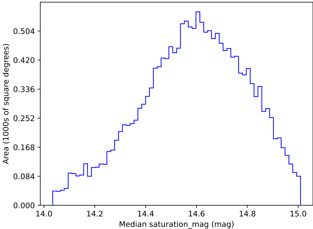
too_elab_r16_d3_giz_v3.4_10yrs WFD g band: Median saturation_mag
