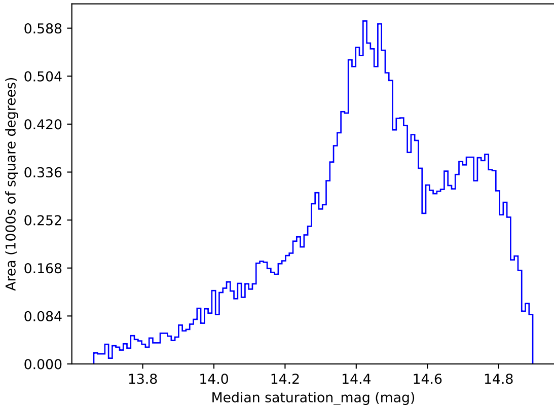
too_elab_r16_d3_giz_v3.4_10yrs All sky i band: Median saturation_mag
