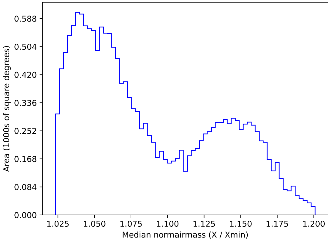
too_elab_r16_d3_giz_v3.4_10yrs WFD z band: Median normairmass
