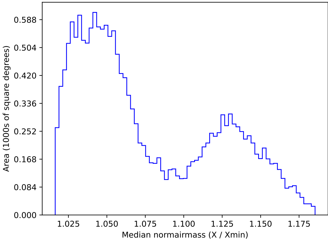
too_elab_r16_d3_giz_v3.4_10yrs WFD r band: Median normairmass
