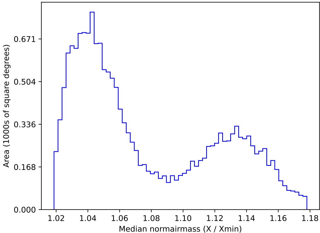
too_elab_r16_d3_giz_v3.4_10yrs WFD i band: Median normairmass
